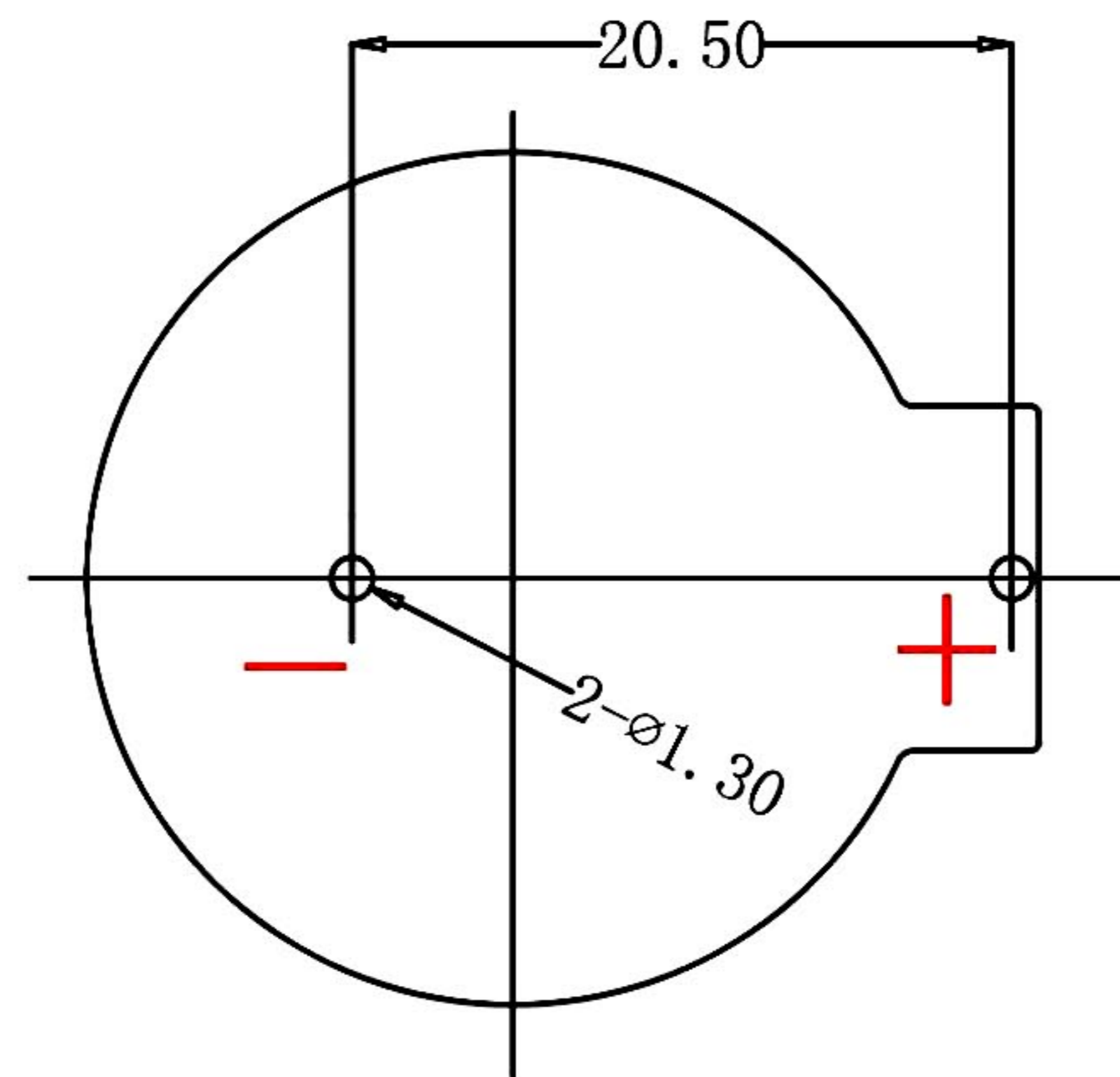
PCB Layout Diagram Top View
