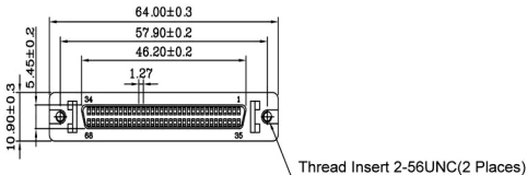
Metal Shell W/ Front Latch
