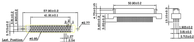
Metal Shell W/ Front Latch
