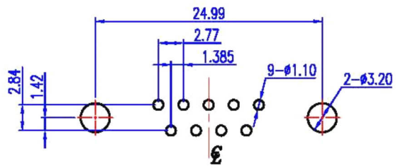
RECOMMENDED P.C.B LAYOUT INSPECTION DIMENSION:(A)~(F)
