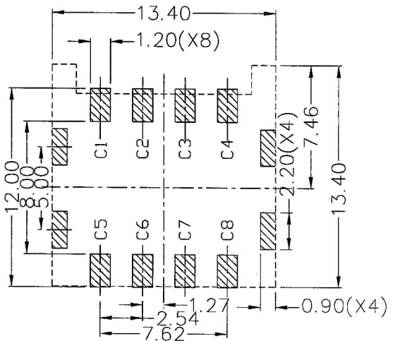
RECOMMENDED P.C.B LAYOUT COMPONENT SIDE(TOLERANCE ±0.05)
