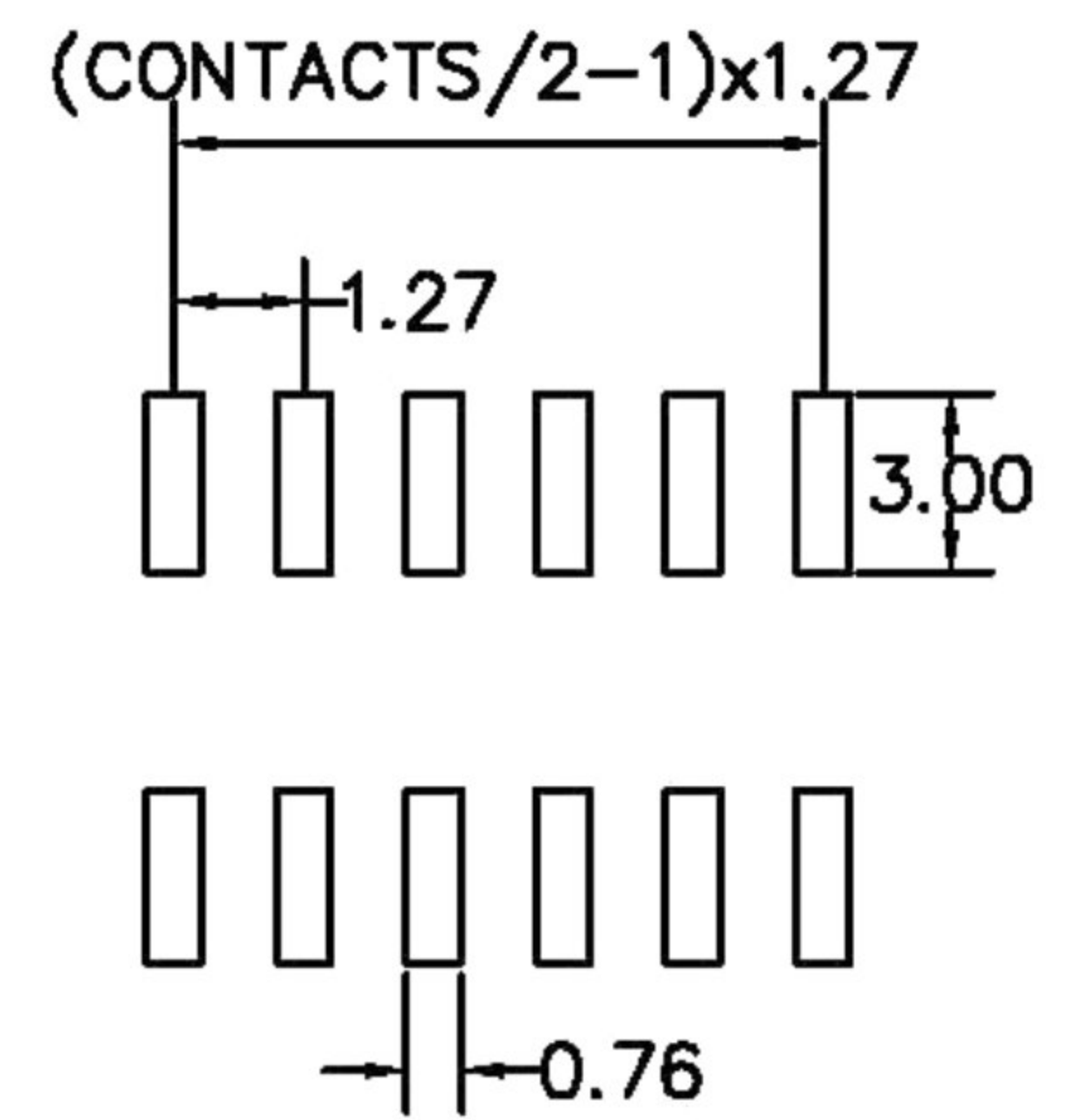
RECOMMENDED P.C.B LAYOUT
