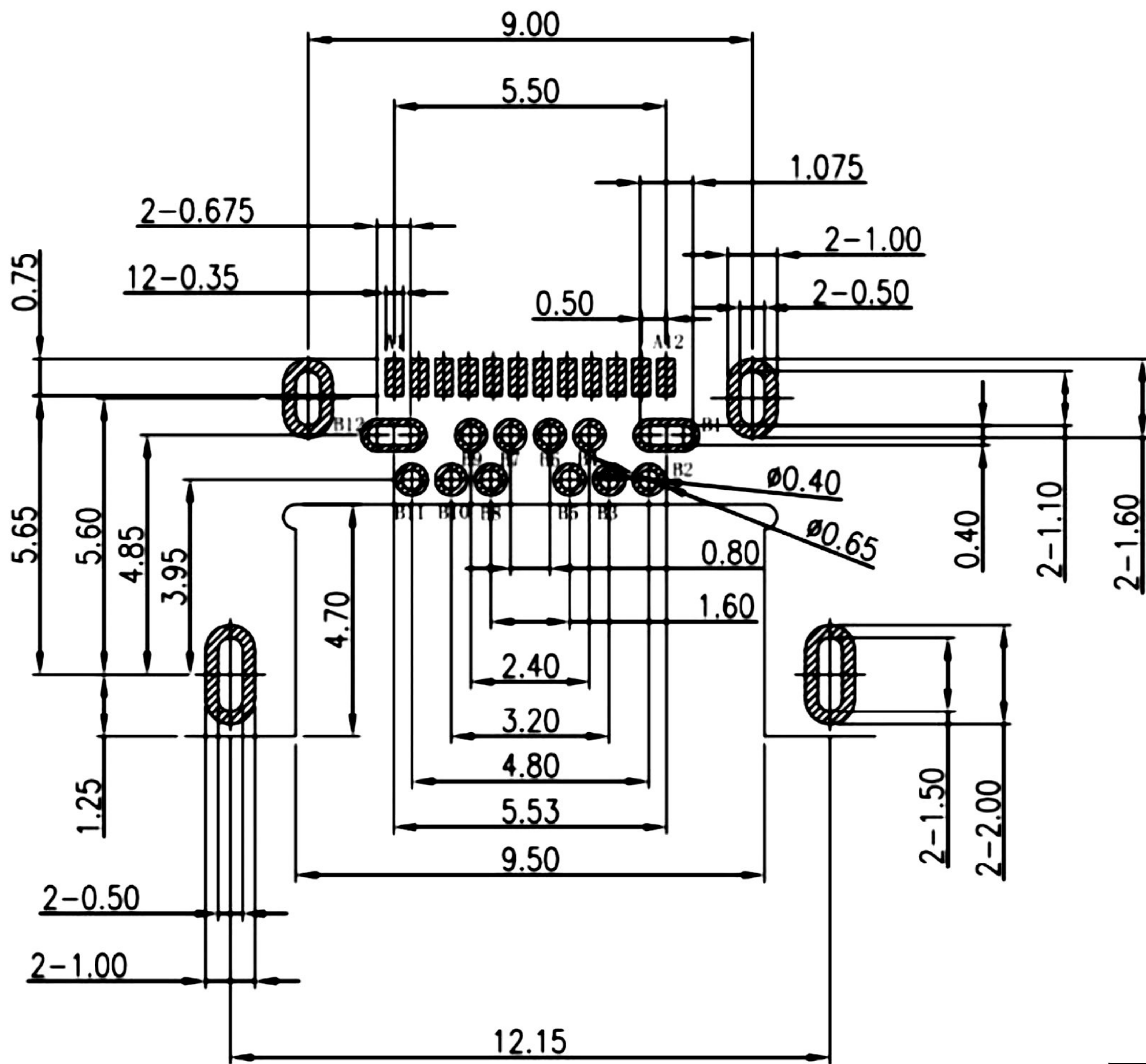
RECOMMENDED P.C.B LAYOUT(Both sides are sample)
