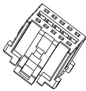
4X2~5X2 3D VIEW
