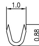
B-B SECTION
